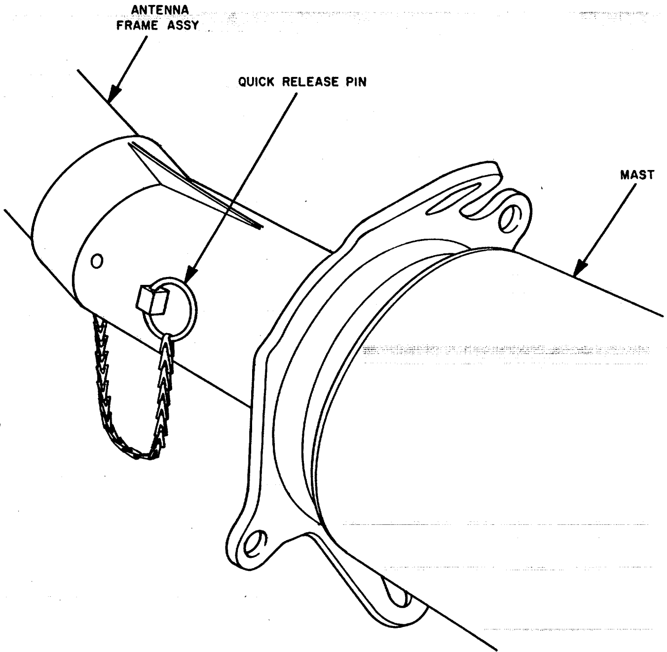
■ Figure 2-5.1. Antenna mounting secured. (B)
